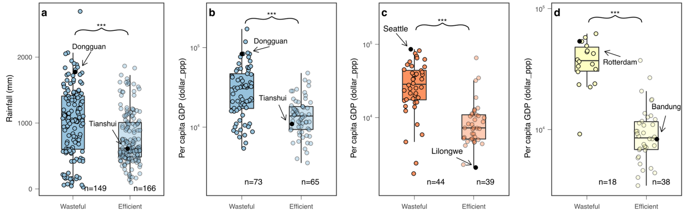
Extended Data Fig. 4 | Comparison of city properties between the wasteful and efficient cities. (a) Cities that produce more wastewater on average feature higher annual rainfall (1030 mm vs. 767 mm, Welch's t -test, p < 0.001 ). (b) Cities that generate more wastewater on average feature higher per capita GDP ($27164 vs. $13312, p < 0.001 ). (c) Cities that generate more municipal solid waste feature
